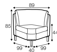
corner 30°
