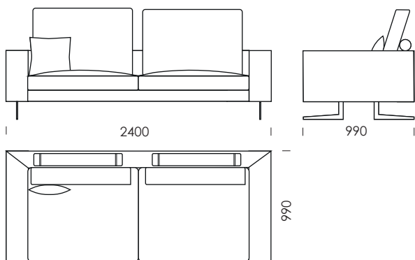
Sofa 3
